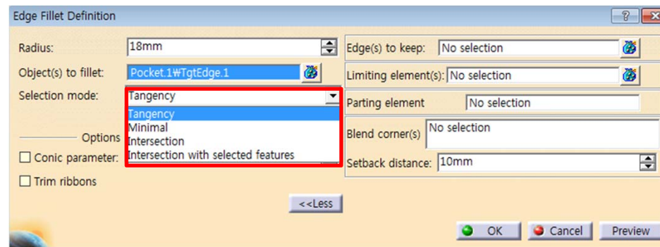
<Tangency>
