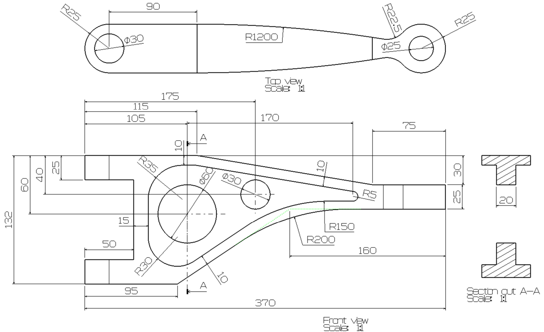
Cantilever
