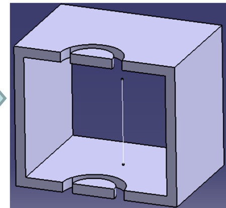
<Merge Ends(Thick)>
