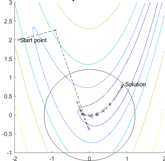
SQP Method on Nonlinearly Constrained Rosenbrock's Function
